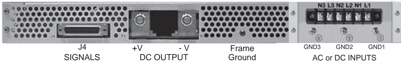
TPCPR1U3B - IEC60320-C20 Input (for use with TPCP, RPCP & RPCQ models)
