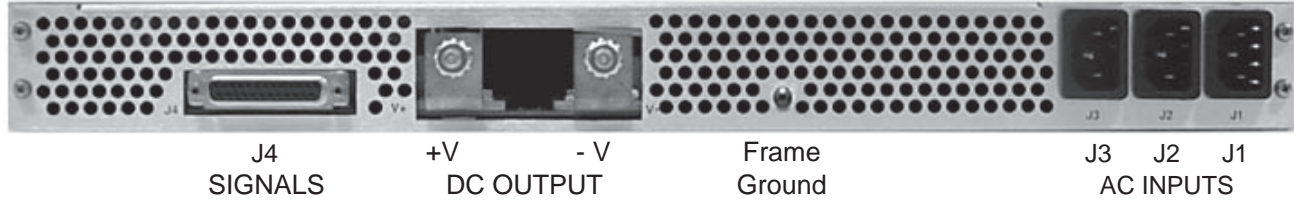
TPCMR1U3E - AC input via module front panel (for use with TPCM3000E, TPCM5000E & TPCM7000E)
