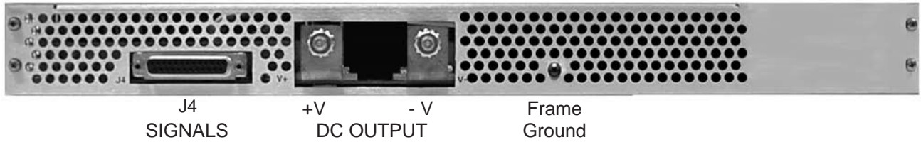
TPCPR1U3A - Screw Terminal Input (for use with TPCP, RPCP & RPCQ models)
