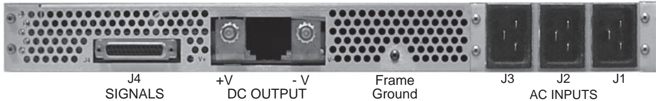
TPCPR1U3C - IEC60320-C20 Filtered Input (for use with TPCP, RPCP & RPCQ models)
